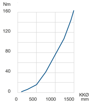
Rotational resistance
